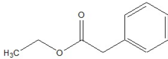
Ethyl phenylacetate
